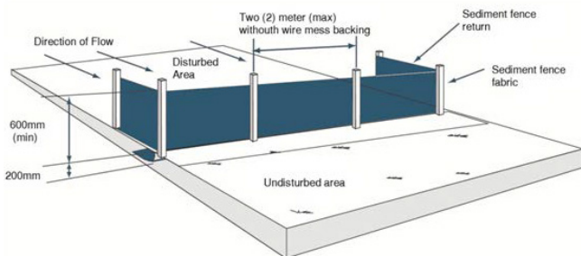
Figure 4: Typical sediment fence installation.
